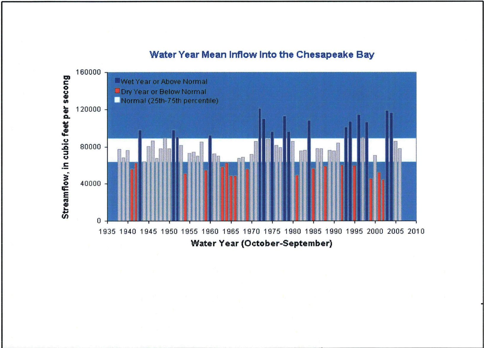
Figure 2.3-9—{Mean Annual Freshwater Inflow in the Chesapeake Bay}
