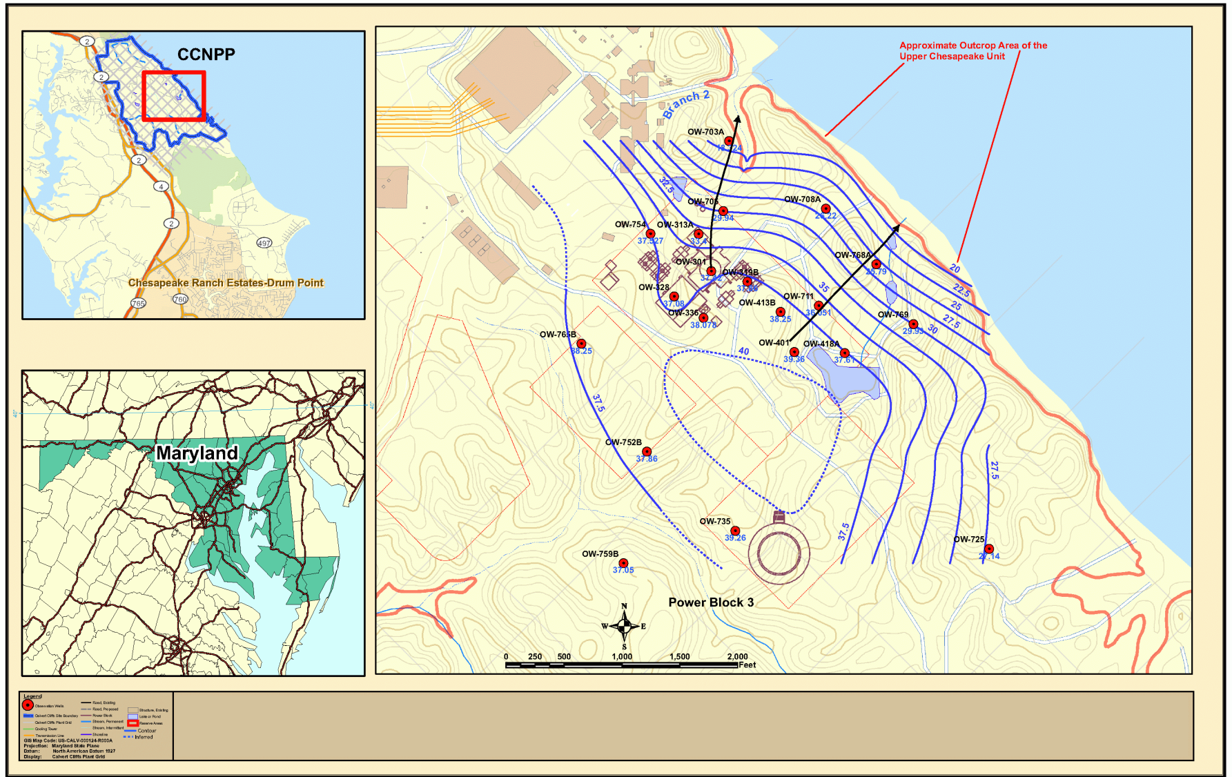
Figure 2.3-47—Potentiometric Surface Elevation Map and Groundwater Flow Directions for the Upper Chesapeake Unit, July 2006
