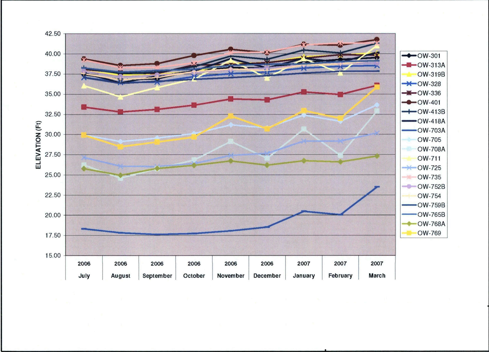
Figure 2.3-46—Groundwater Elevations for the Upper Chesapeake Unit, July 2006 through March 2007
