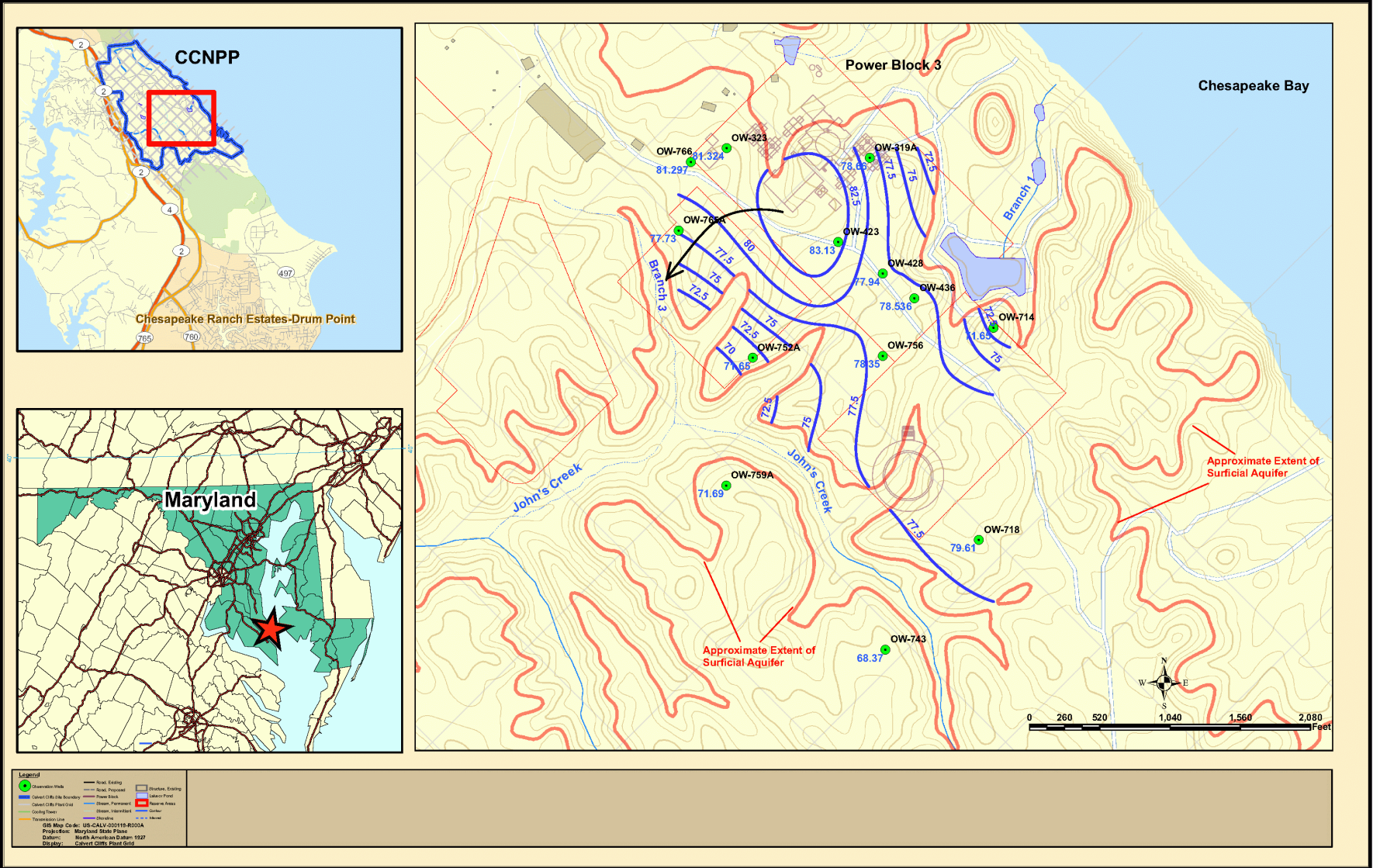
Figure 2.3-43—Water Table Elevation Map and Groundwater Flow Direction for the Surficial Aquifer, September 2006
