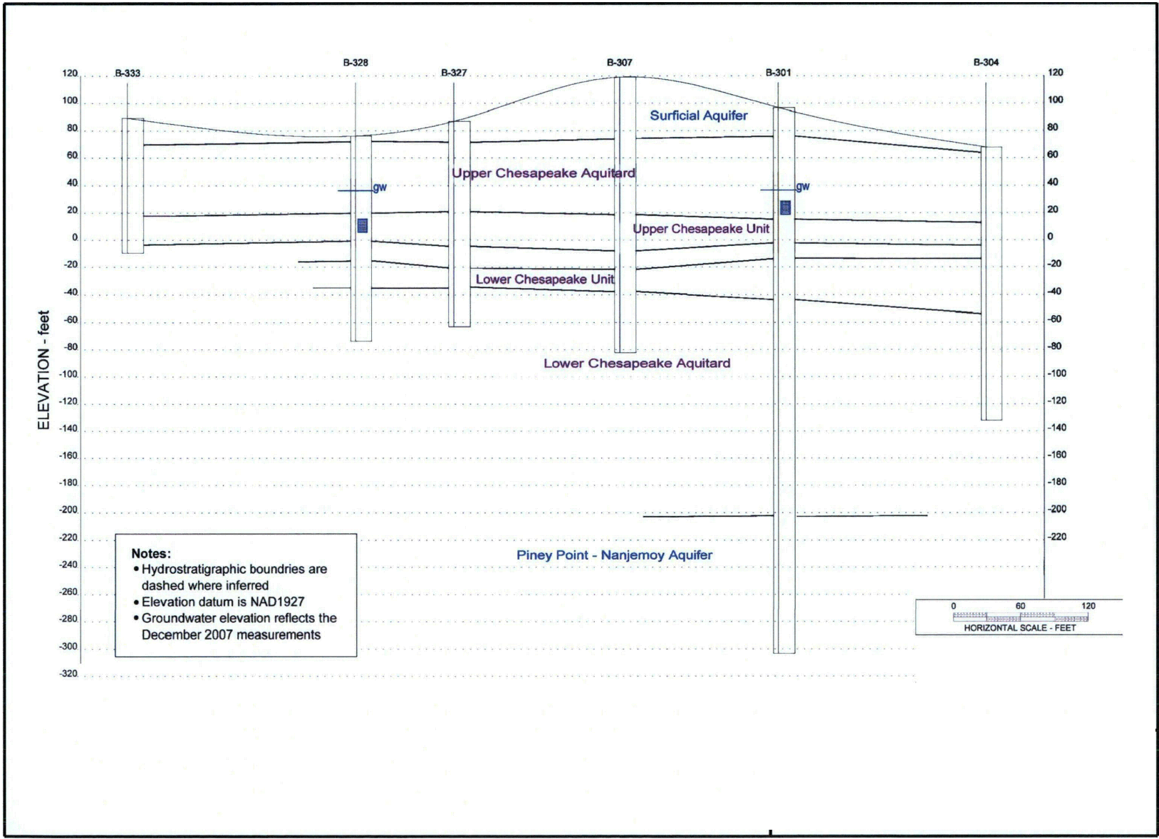
Figure 2.3-39—{Cross Section B-B' through Proposed Unit 3 Power Block Area}
