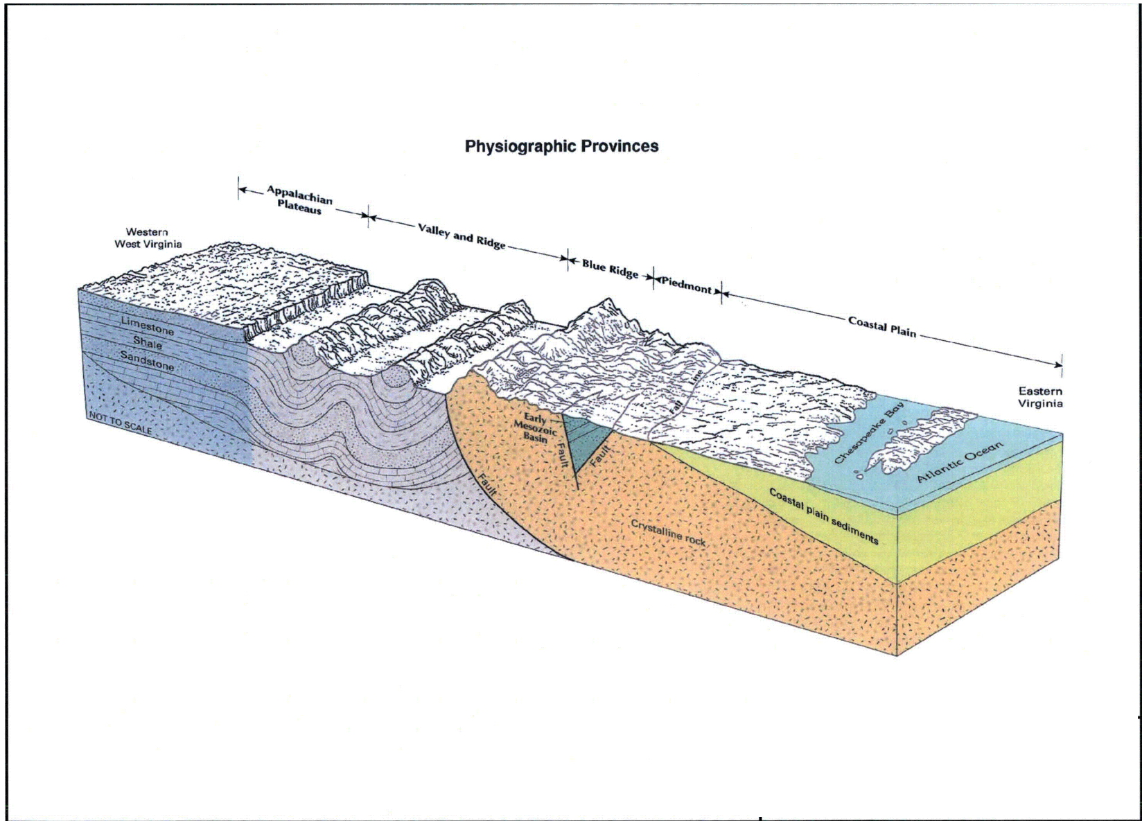
Figure 2.3-30—{Schematic Geologic Cross Section through the Mid-Atlantic Region}
