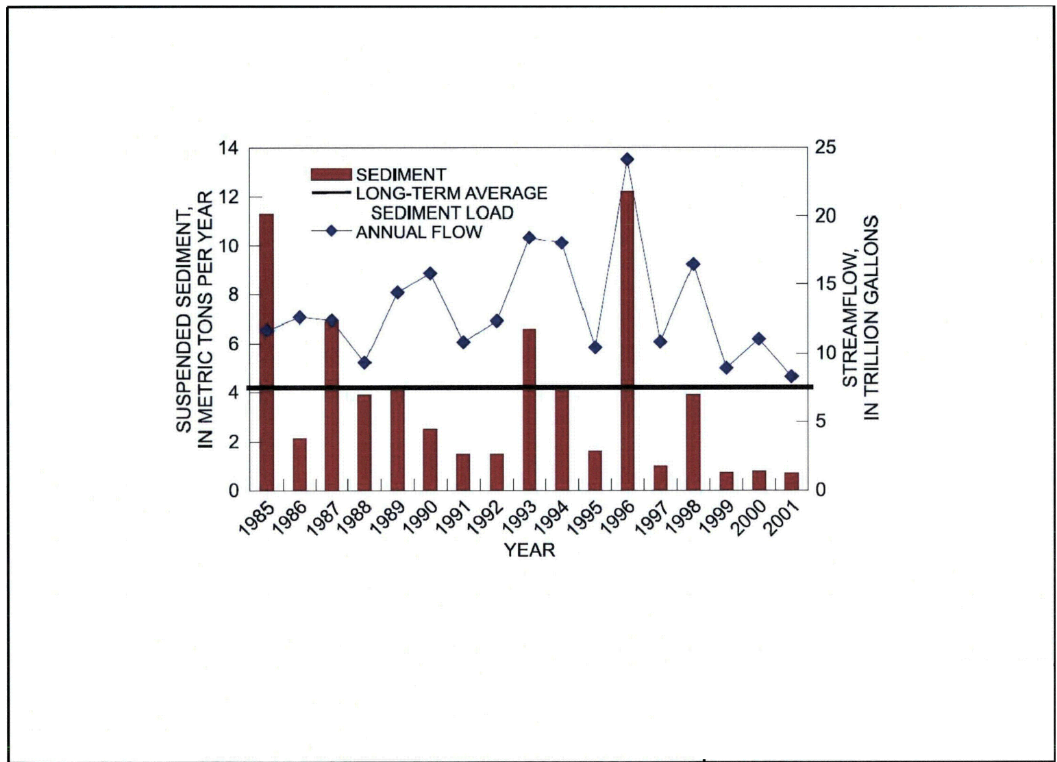
Figure 2.3-24—{Combined Annual Suspended Loads and Relation to Annual Flow from the Susquehanna, Potomac and James Rivers near the Fall Line}
