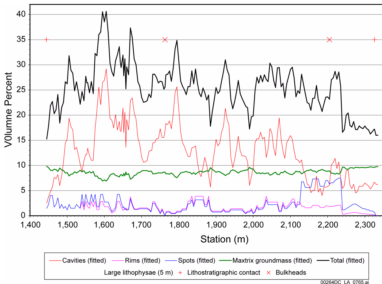
Figure 2.3.4-25. Calculated Porosity of Lithophysal Cavities, Rims, Spots, Matrix Groundmass, and the Total Porosity in the Tptpl Exposed along the Enhanced Characterization of the Repository Block Cross-Drift
