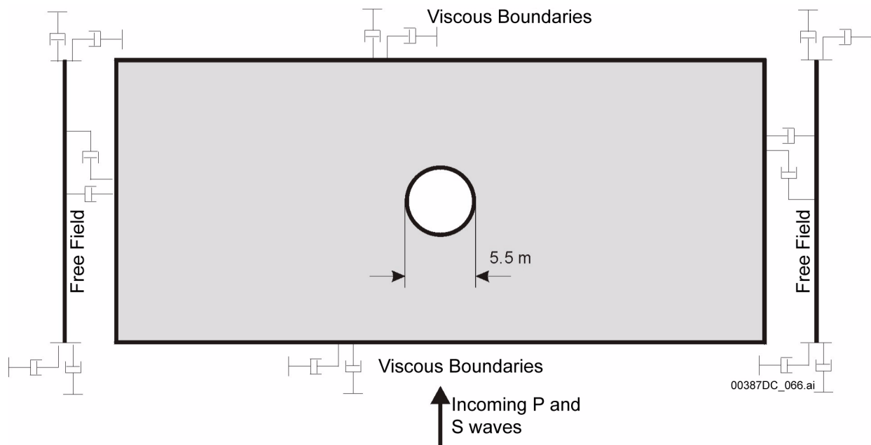
Figure 2.3.4-36. Schematic of Model Boundary Conditions for Dynamic Simulation
