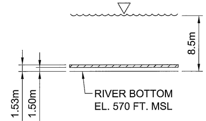
CROSS SECTION SHOWING PLUME DEPTH WATER SURFACE LEVEL = 598 FT. MSL RIVER TEMP. = 32.2°C
