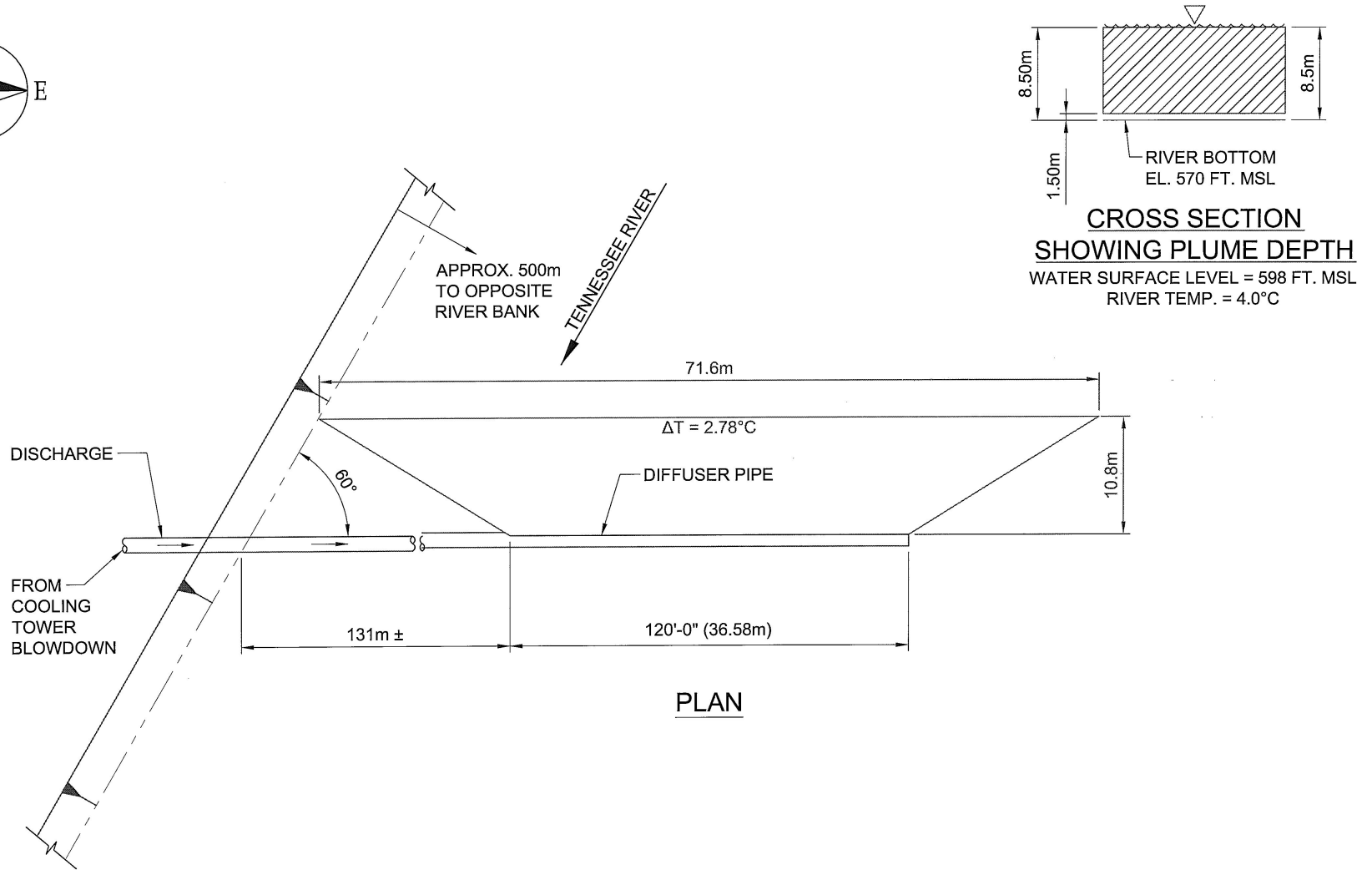
FIGURE 5.3-9 Low River Temperature, Maximum Reverse River Flow
