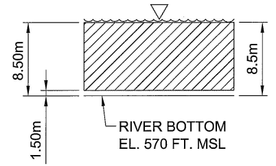
CROSS SECTION SHOWING PLUME DEPTH WATER SURFACE LEVEL = 598 FT. MSL RIVER TEMP. = 32.2°C
