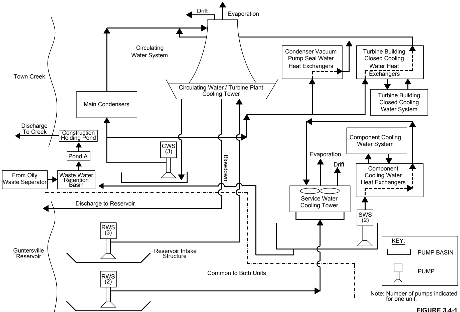
FIGURE 3.4-1 General Cooling System Flow Diagram
