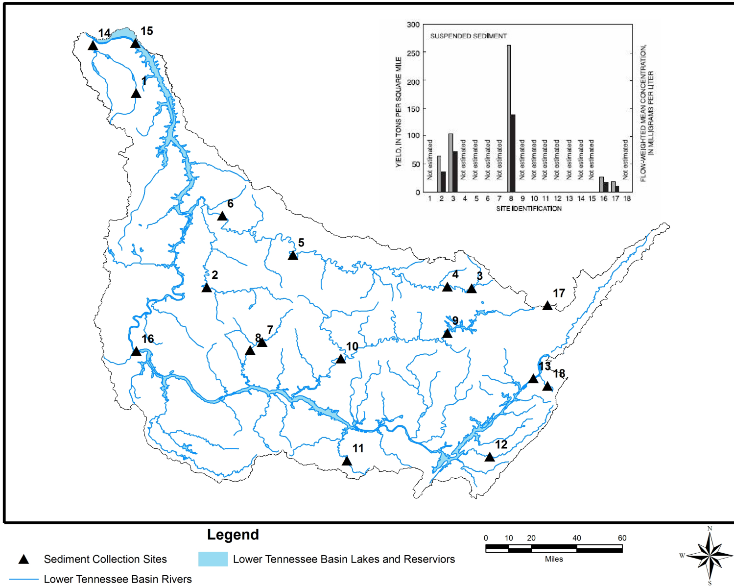
FIGURE 2.3-8 Annual Yield and Flow-Weighted Mean Concentration of Suspended Sediment at Selected Sites in the Lower Tennessee River Basin
