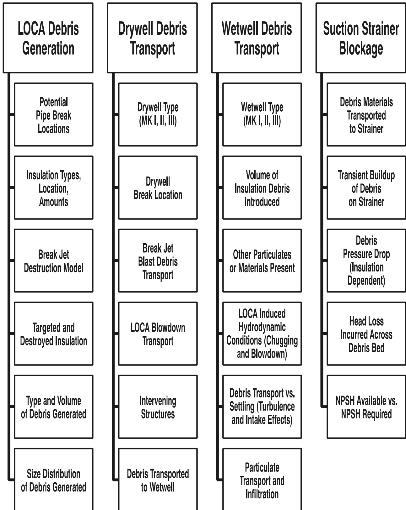
Figure 4. Debris Blockage Considerations for BWR LOCA Sequences
