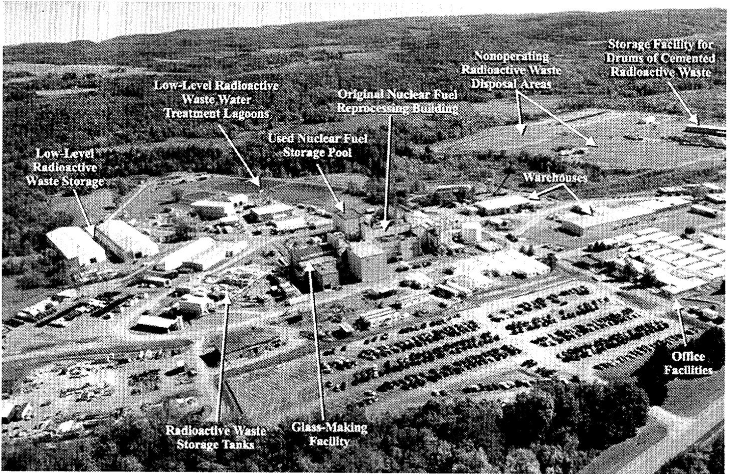
Figure 1: Aerial View of the West Valley Site During DOE Operations
