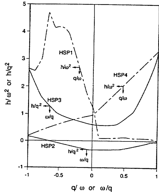
Fig. 4-11. Semiscale two-phase fully degraded homologous pump-head curves.
